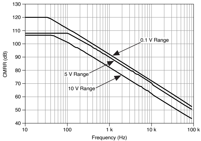
Figure 3. AI <0..31> CMRR
